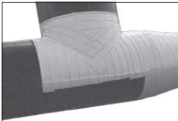
Stopaq CZ tape for complicated pipeline parts DVGW approved to DIN 30672/EN 12068 class A/30
